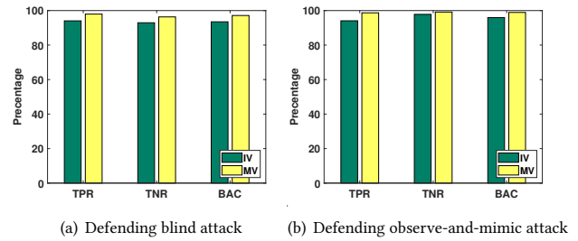
Figure 14: Authentication performance on defending blind attack and observe-and-mimic attack.
